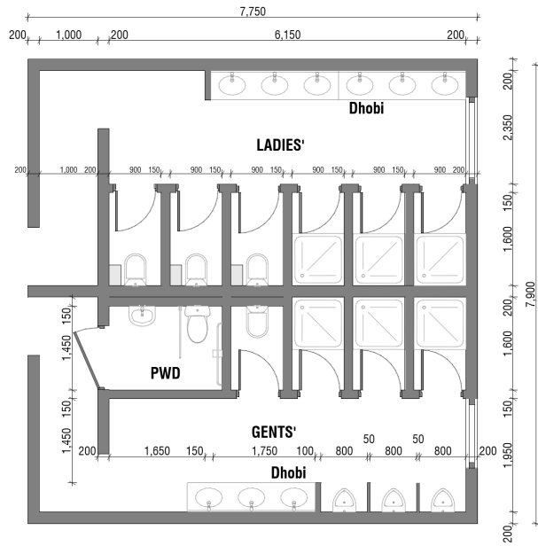
Shared washrooms GROUND FLOOR
