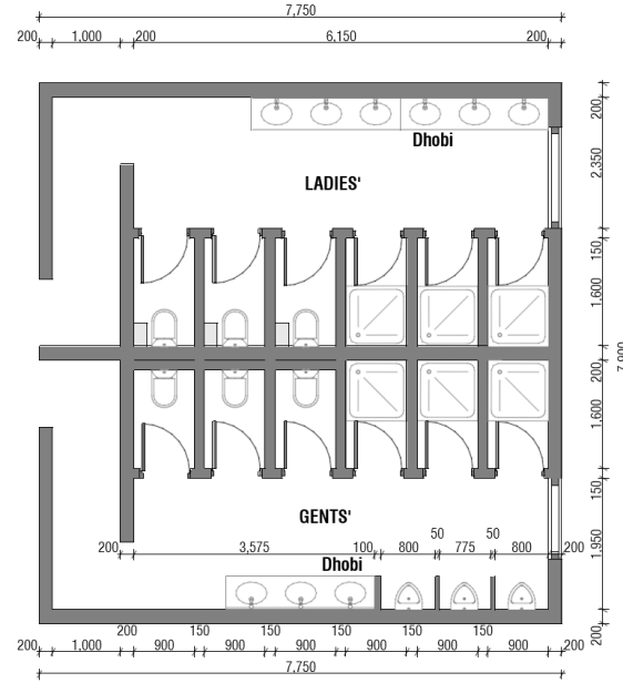
Shared washrooms TYPICAL FLOORS
