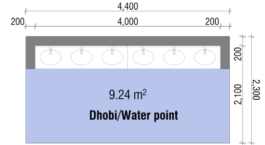
Shared Dhobi TYPICAL FLOORS
